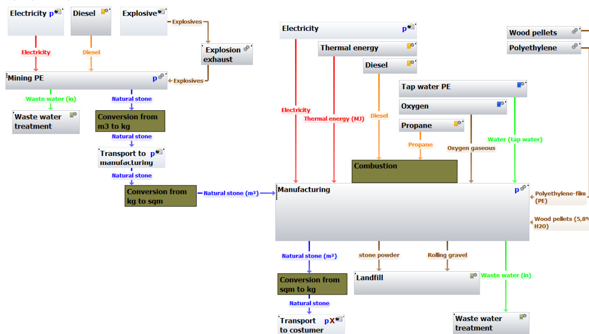
Massive slabs from hard rock - 1 tonne GaBi 5 process plan: Reference quantities
